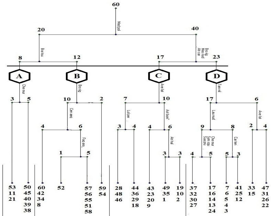
Fig. 3. Two Way Indicator Species Analysis (TWINSPAN) dendrogram of the 60 sampled stands based on the importance values of the 84 species. The indicator species are abbreviated by the first three letters of genus and species respectively.
